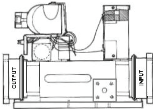
Multipactor FIGURE 10
