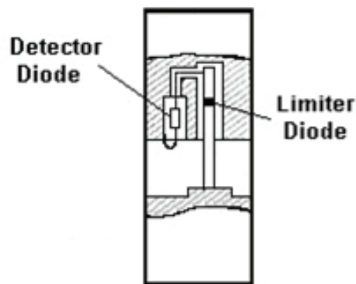
Diode Limiter FIGURE 11
