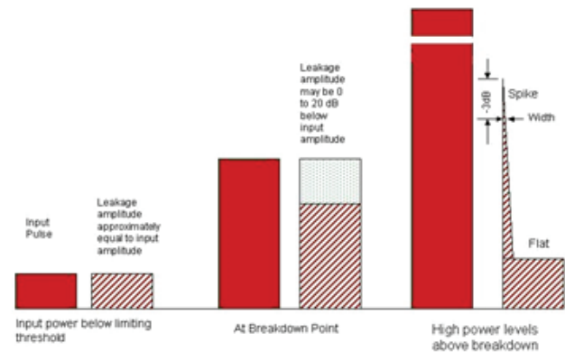
Input - Output Characteristic Waveforms FIGURE 5
